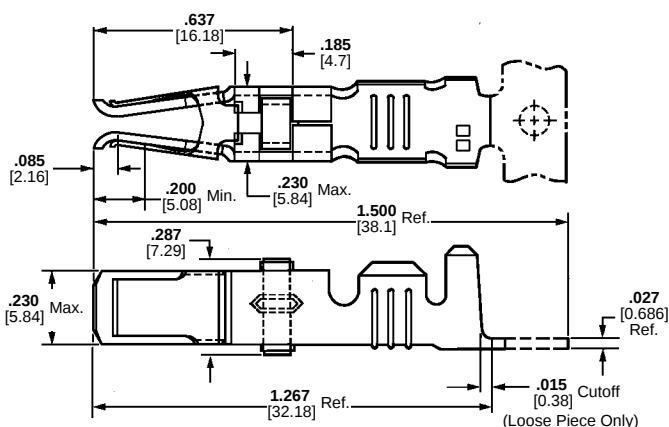
Female
