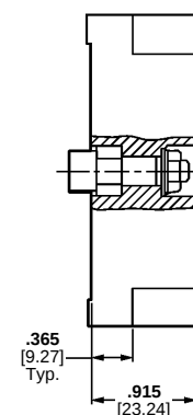
Receptacle Housing Phenolic Part No. 202800-2 Diallyl Phthalate Part No. 202800-1
