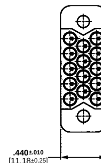
Receptacle Assembly
