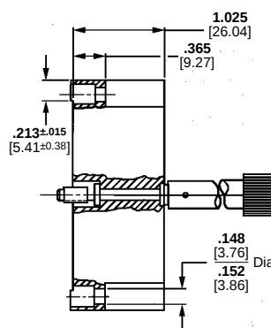
Plug Housing
