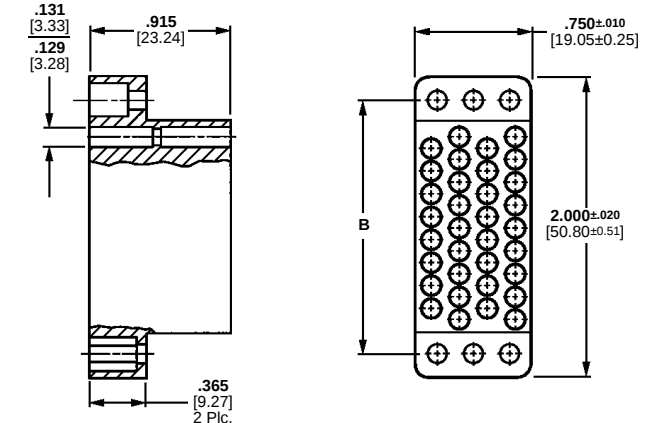
Plug Housing (Shown)
