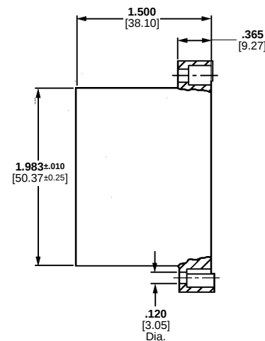
Receptacle Housing
