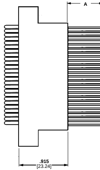
Plug Assembly
