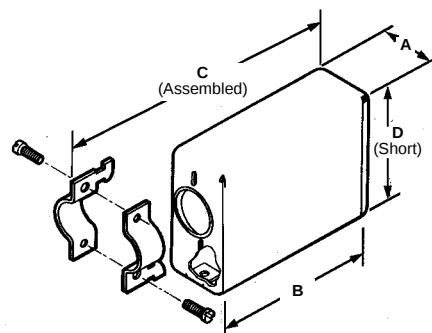
90° Cable Exit
