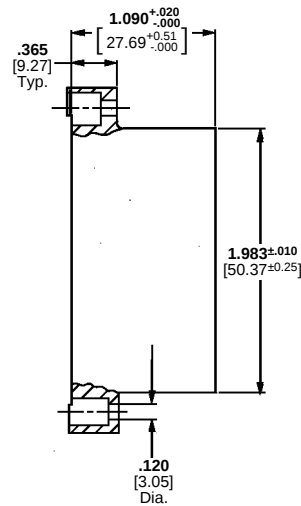
Plug Housing
