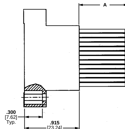
Receptacle Assembly
