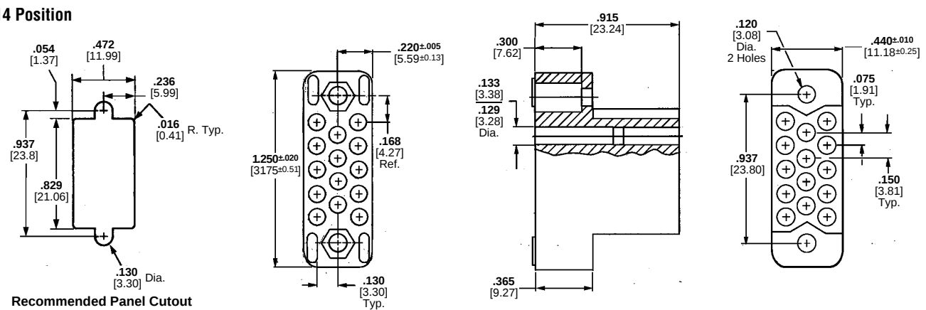
Recommended Panel Cutout
