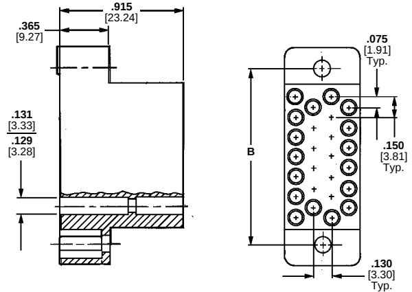
Plug Housing (Shown)
