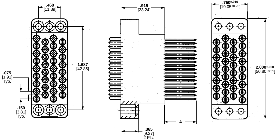
Plug Assembly
