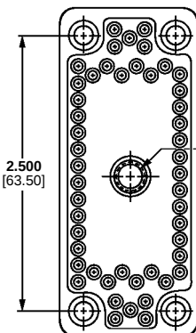
Receptacle Housing
