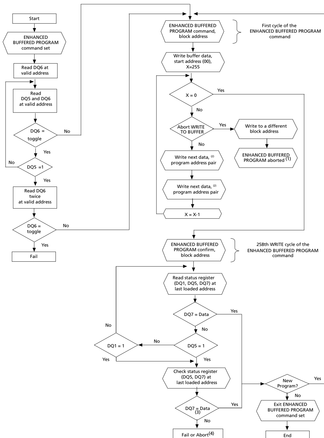
Figure 10: ENHANCED BUFFERED PROGRAM Flowchart
