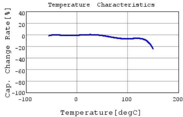
RHEL82A153K0M1H03A C-Temp. capchange, DCOV,
