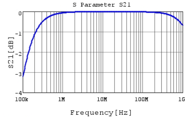
RHEL82A153K0M1H03A S21 DCOV, 25degC
