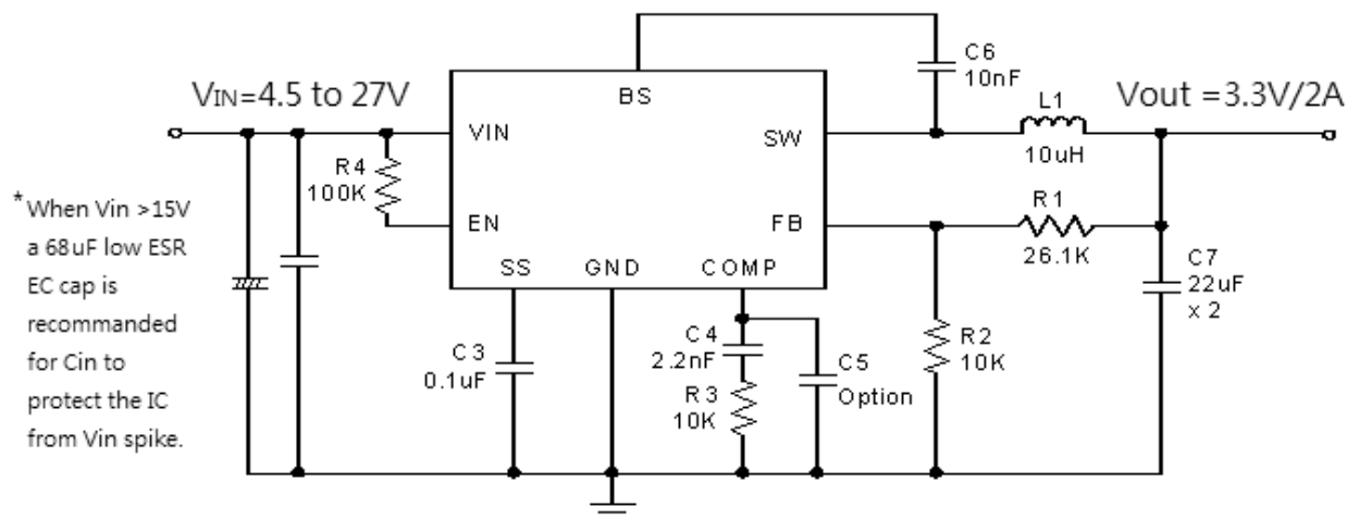
TD8202X Circuit, 3.3V/2A output
