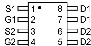
pin assignment
