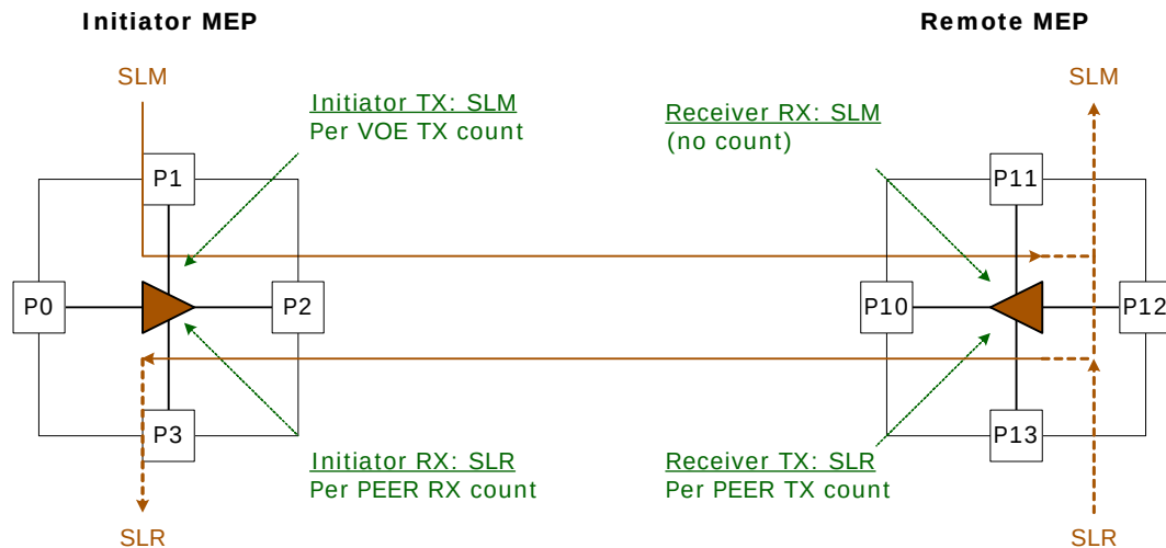
Figure 74 • Single-Ended SynLM
