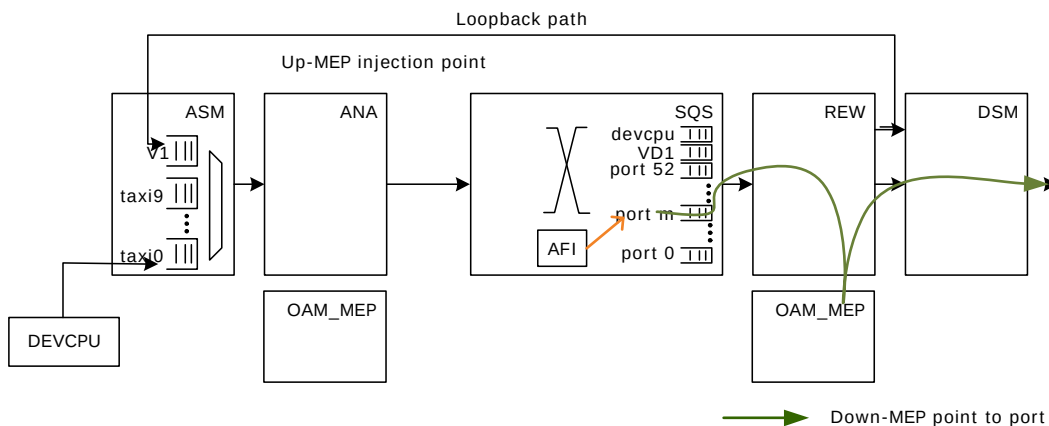
Figure 136 • Down-MEP Injection from AFI
