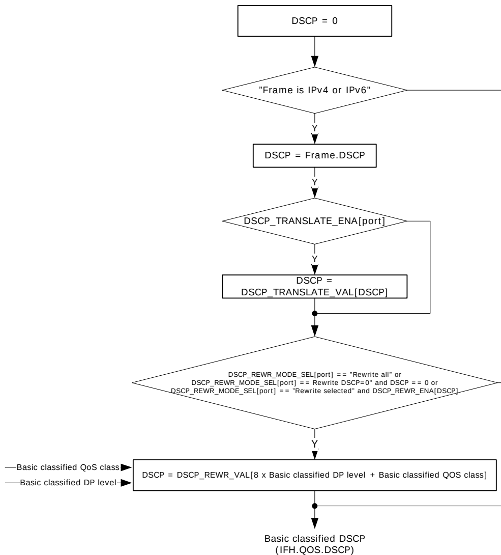
Figure 33 • Basic DSCP Classification Flow Chart
