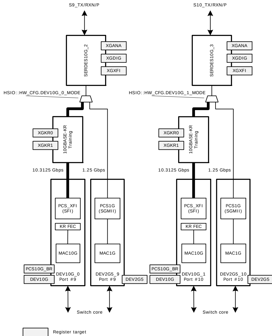
Figure 16 • 10G Muxing
