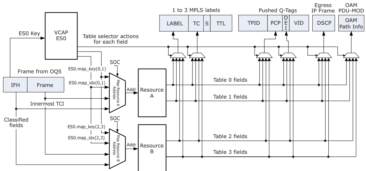
Figure 114 • Mapping Tables
