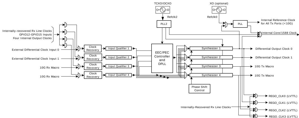
Figure 124 • SyncE Controller
