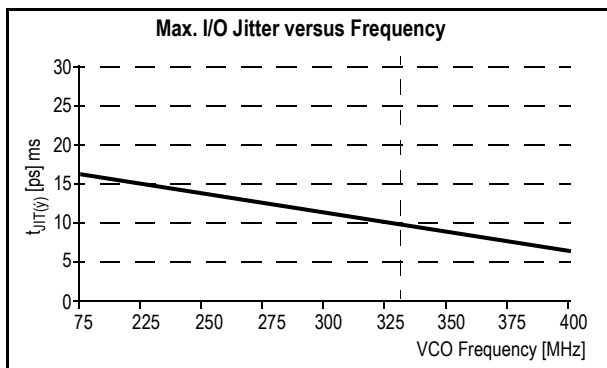
Figure 6. Maximum I/O Jitter (RMS) versus Frequency for V_{CC} = 3.3 V
