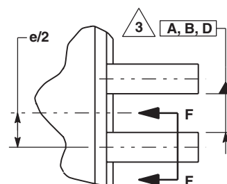
DETAIL G
