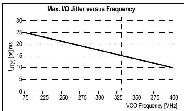
Figure 5. Maximum I/O Jitter (RMS) versus Frequency for V_{CC} = 2.5 V
