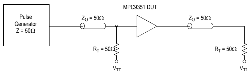
Figure 11. TCLK MPC9351 AC Test Reference for V_{CC} = 3.3\text{ V} and V_{CC} = 2.5\text{ V}
