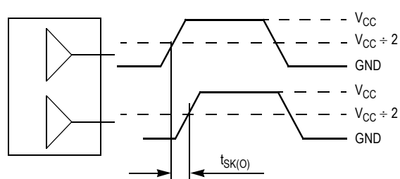
Figure 16. Output-to-Output Skew t_{SK(O)}
