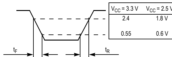
Figure 20. Transition Time Test Reference
