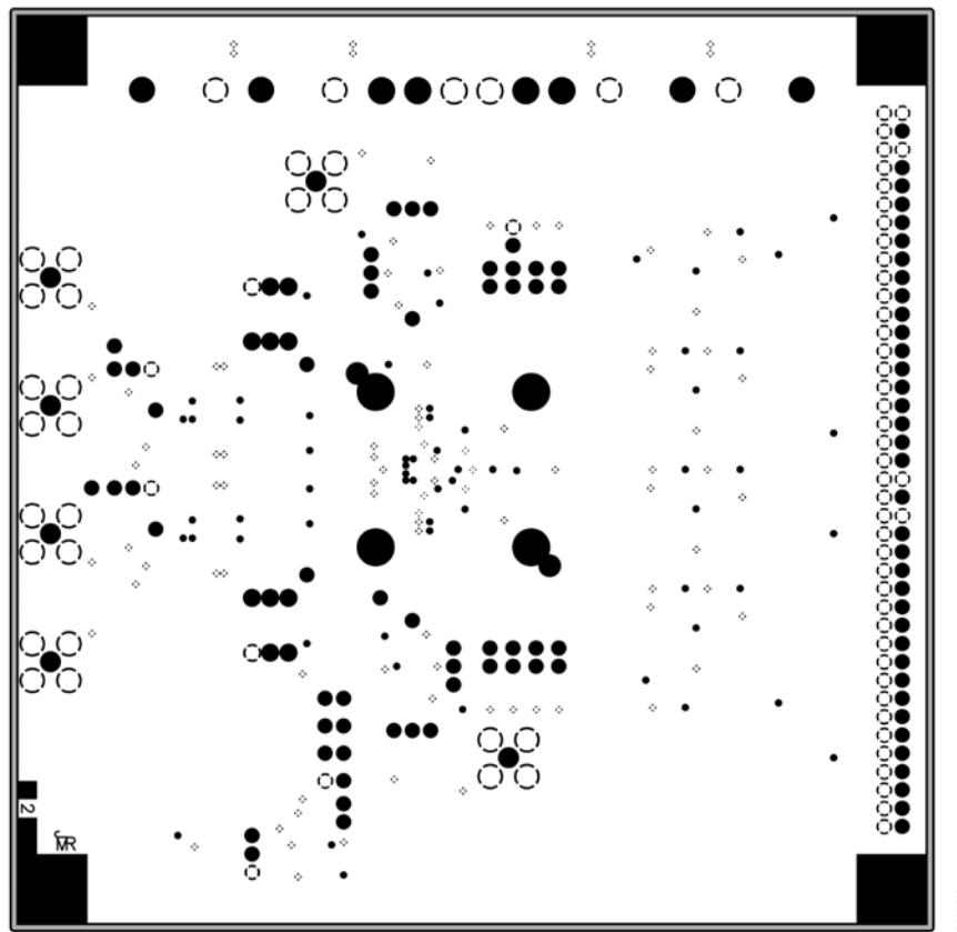
Figure 46. PCB Ground Plane
