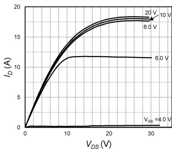
Fig.1 On-Region Characteristics.
