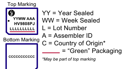
44-Lead PLCC
