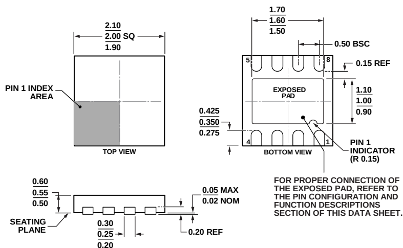
Figure 57. 8-Lead Lead Frame Chip Scale Package [LFCSP_UD] 2.00 mm × 2.00 mm Body, Ultra Thin, Dual Lead (CP-8-10)
