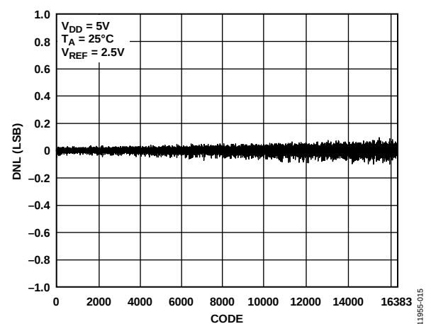
Figure 15. AD5682R DNL
