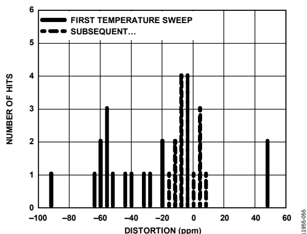
Figure 55. Thermal Hysteresis
