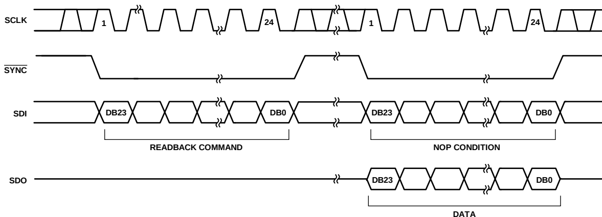
Figure 54. Readback Operation
