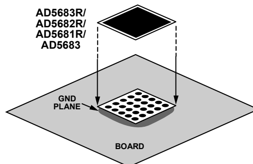
Figure 56. Pad Connection to Board
