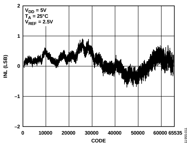
Figure 11. AD5683R/AD5683 INL
