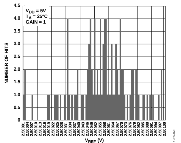
Figure 28. Reference Output Spread
