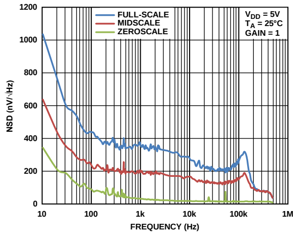
Figure 35. Noise Spectral Density vs. Frequency, Gain = 1
