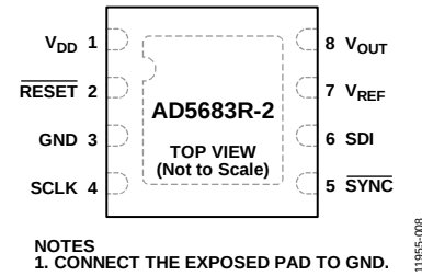
Figure 8. Pin Configuration, 8-Lead LFCSP, RESET Option
