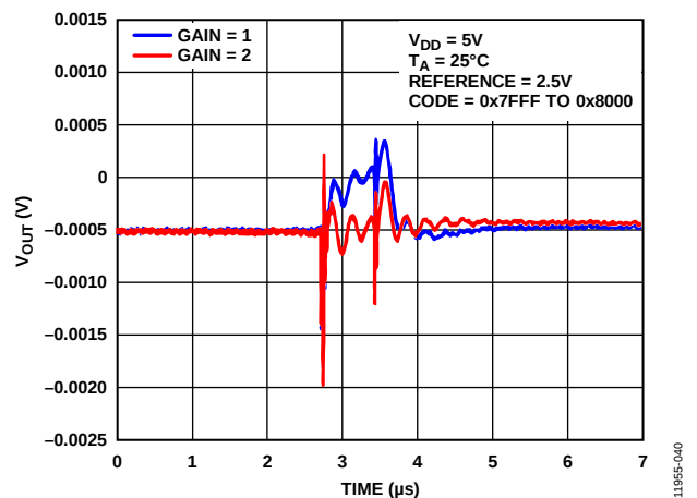
Figure 40. Digital-to-Analog Glitch Impulse
