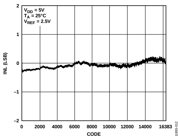
Figure 12. AD5682R INL
