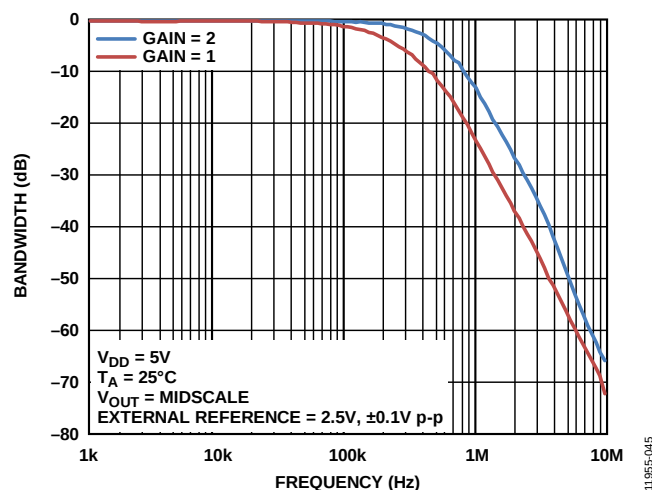
Figure 45. Multiplying Bandwidth, External Reference 2.5\text{ V} \pm 0.1\text{ V p-p} , 10 kHz to 10 MHz
