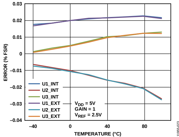
Figure 23. Gain Error and Full-Scale Error vs. Temperature
