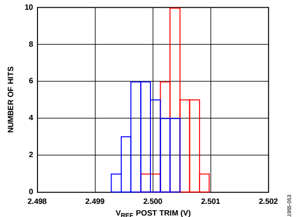
Figure 53. SHR Reference Voltage Shift
