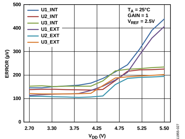
Figure 27. Zero Code Error and Offset Error vs. Supply
