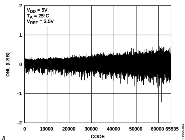
Figure 14. AD5683R/AD5683 DNL
