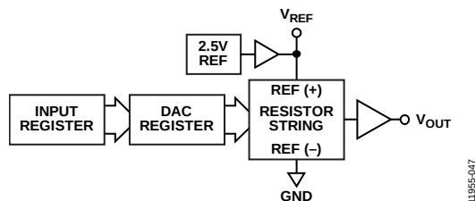
Figure 47. DAC Channel Architecture Block Diagram
