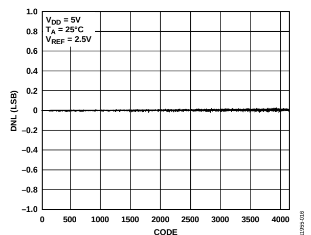
Figure 16. AD5681R DNL
