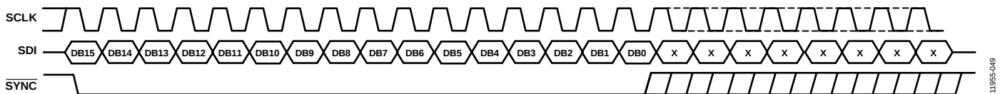
Figure 49. Short Write on the AD5681R
