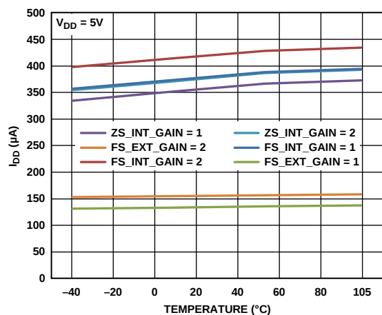
Figure 37. Supply Current vs. Temperature
