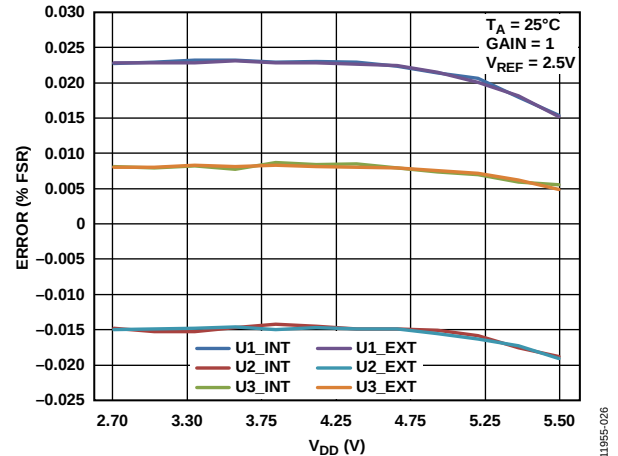
Figure 26. Gain Error and Full-Scale Error vs. Supply
