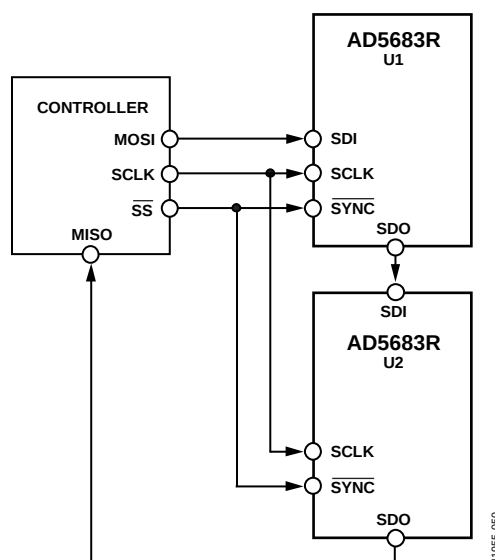
Figure 50. Daisy-Chain Connection
