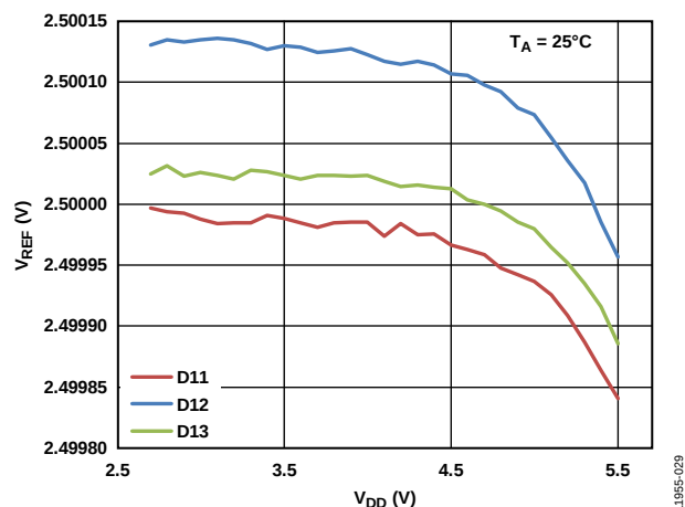
Figure 29. Internal Reference Voltage vs. Supply Voltage
