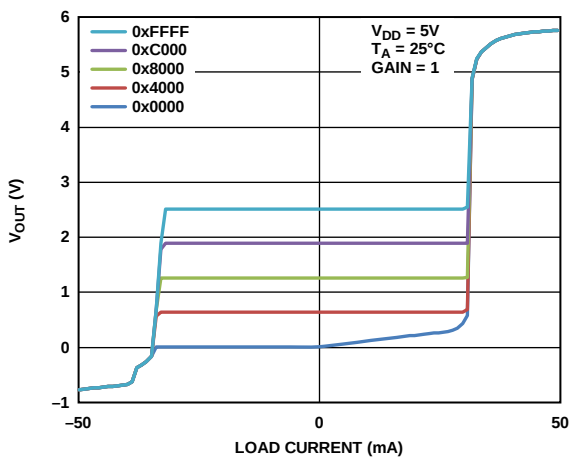
Figure 36. Source and Sink Capability, Gain = 1
