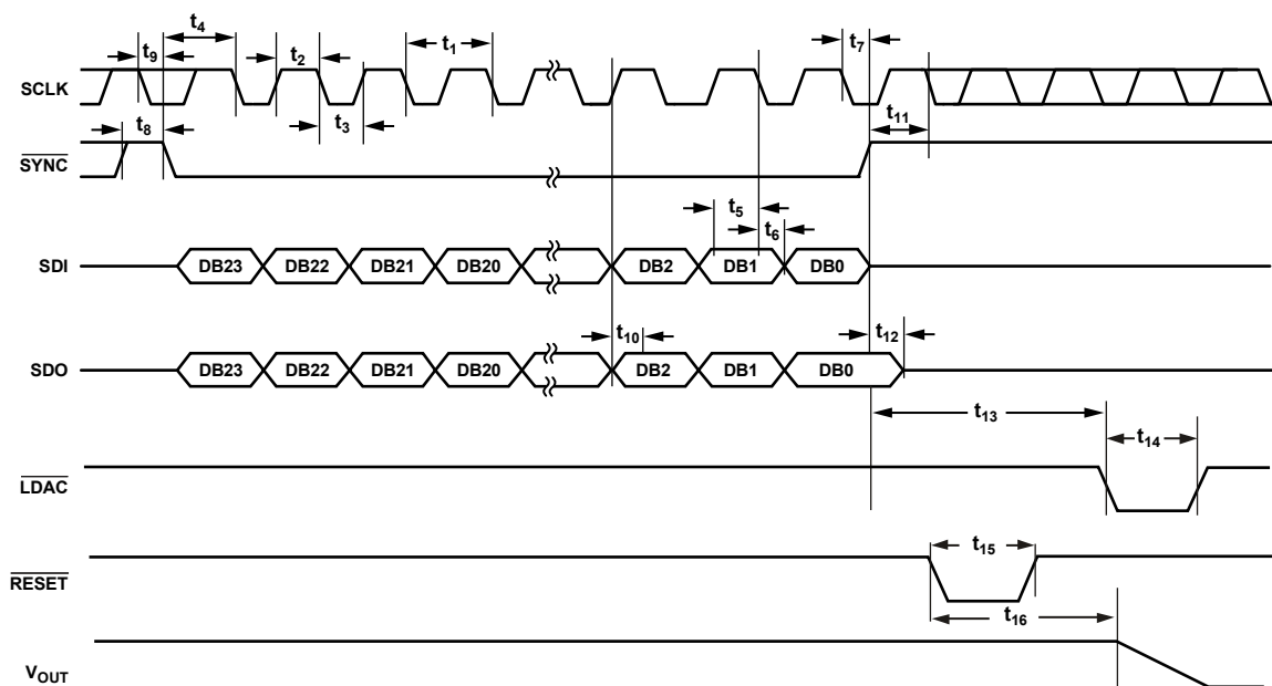
Figure 4. SPI Timing Diagram, Compatible with Mode 1 and Mode 2 (See the AN-1248 Application Note )
