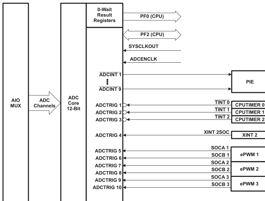
Figure 6-3. ADC Connections
