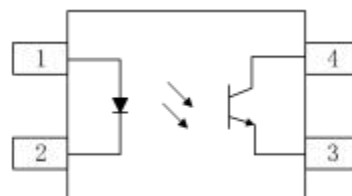
Pin Configuration
