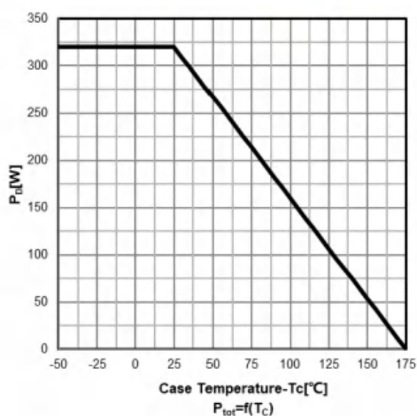
Power dissipation
