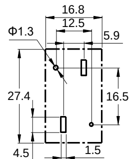
Reference Hole Pattern
