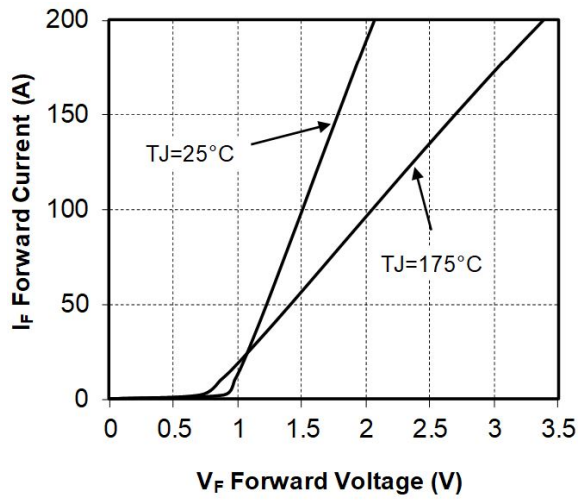
Figure 1-16. Forward Characteristics
