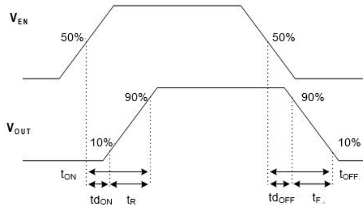
Timing Diagram
