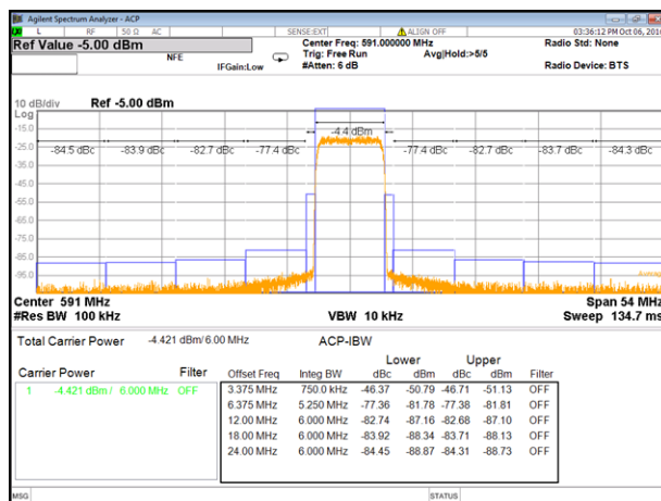
Figure 144. ACPR Performance of 6 MHz Single Carrier at 591 MHz
