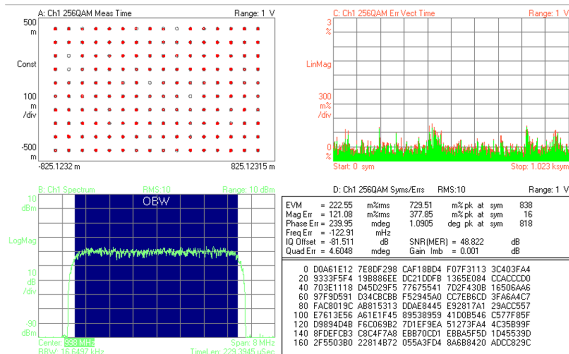
Figure 147. Unequalized MER of 6 MHz Single Carrier at 998 MHz
