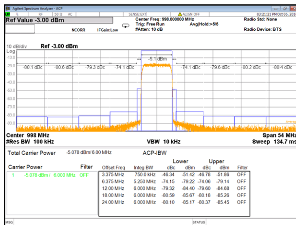
Figure 145. ACPR performance of 6 MHz Single Carrier at 998 MHz
