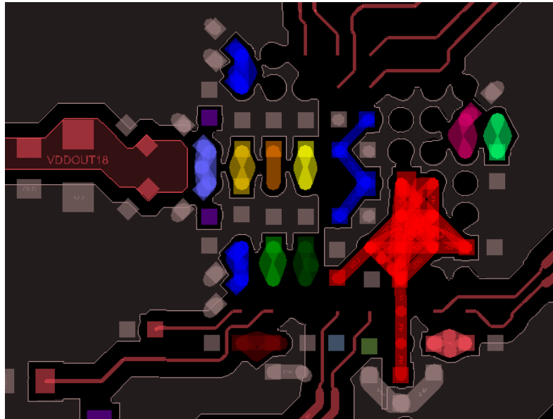
Figure 150. Bypass Capacitors Placed on the Power Supply Pin With In-pad Vias
