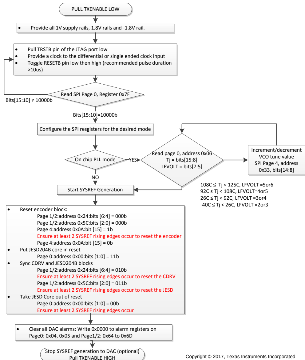
Figure 141. DAC38RF82/89 Recommended Startup Sequence
