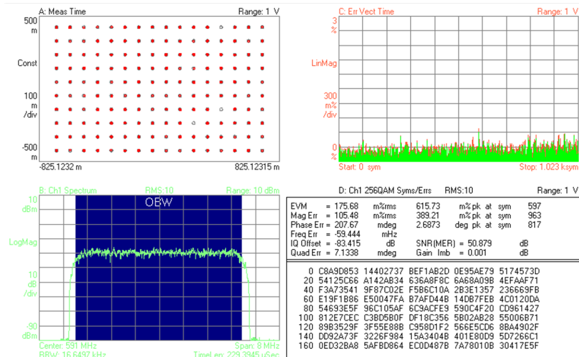
Figure 146. Unequalized MER of 6 MHz Single Carrier at 591 MHz
