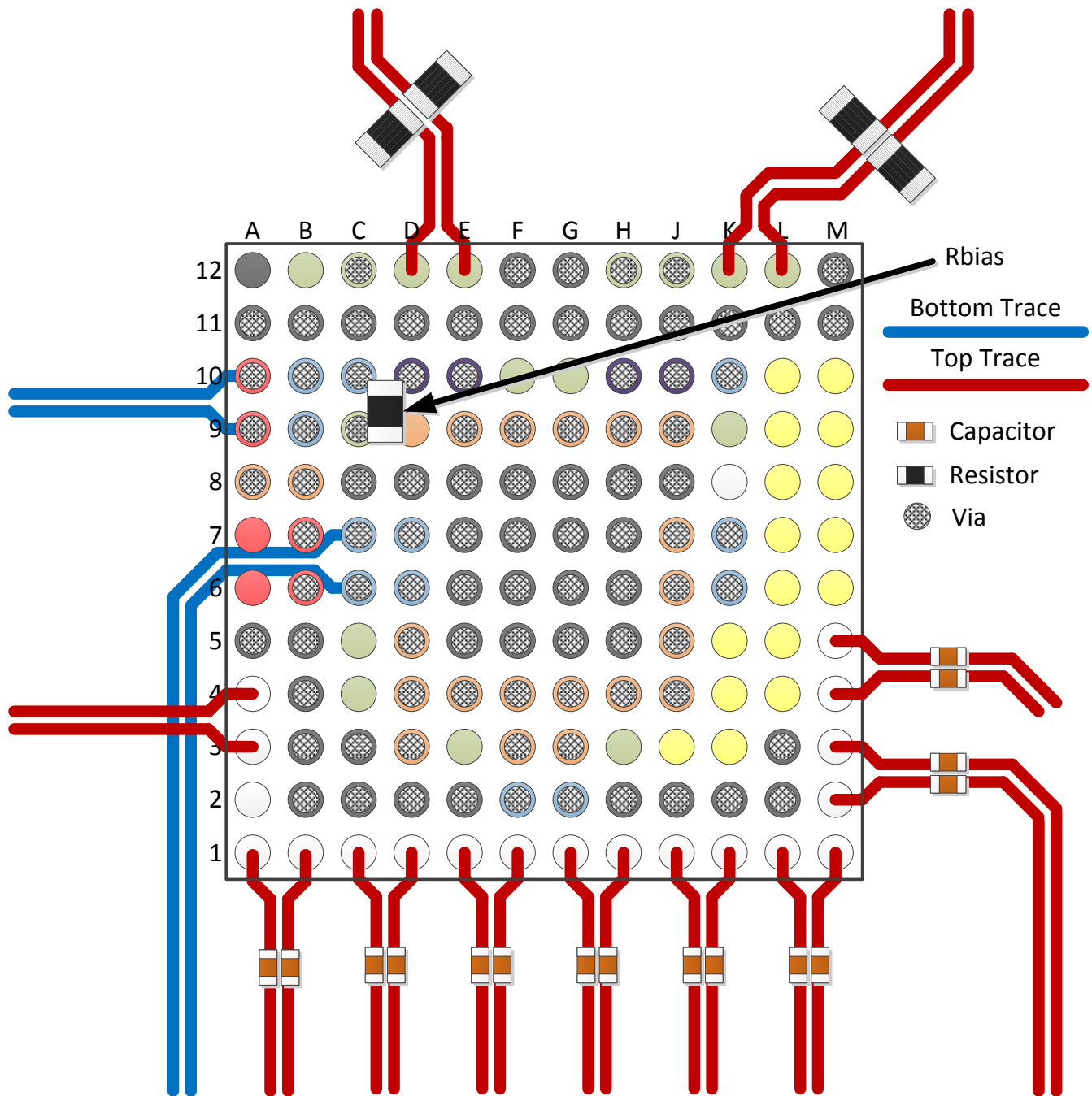
Figure 152. Layout Example
