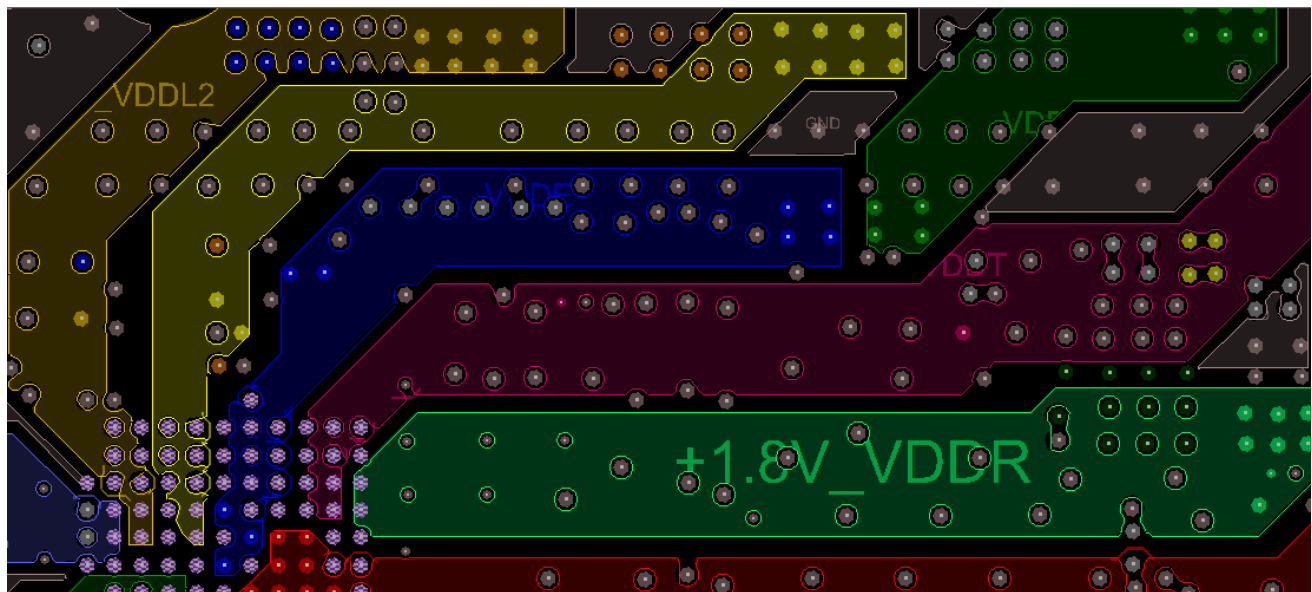
Figure 149. Example Power Plane Routing
