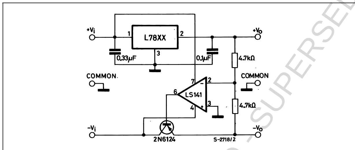
Figure 21 : Split Power Supply ( \pm 15\text{V} - 1\text{ A} )
