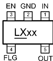
MIC5256-x.xYM5 5-Pin SOT23
