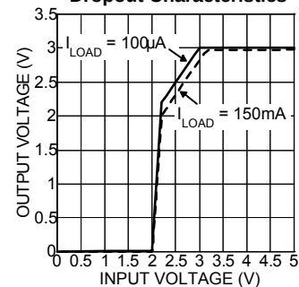
Dropout Characteristics
