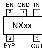
MIC5256-x.xYD5 5-Pin Thin SOT23
