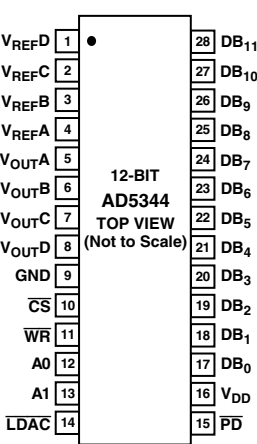
AD5344 PIN CONFIGURATION
