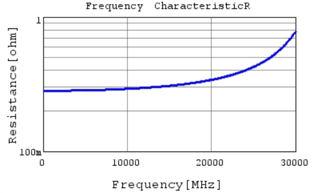
GJM0335C2AR70BB01 R DCOV, 25degC
