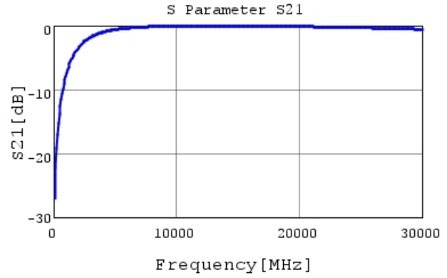
GJM0335C2AR70BB01 S21 DCOV, 25degC
