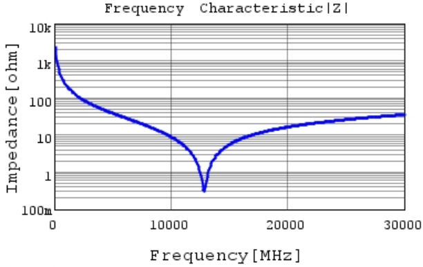
GJM0335C2AR70BB01 |Z| DCOV, 25degC
