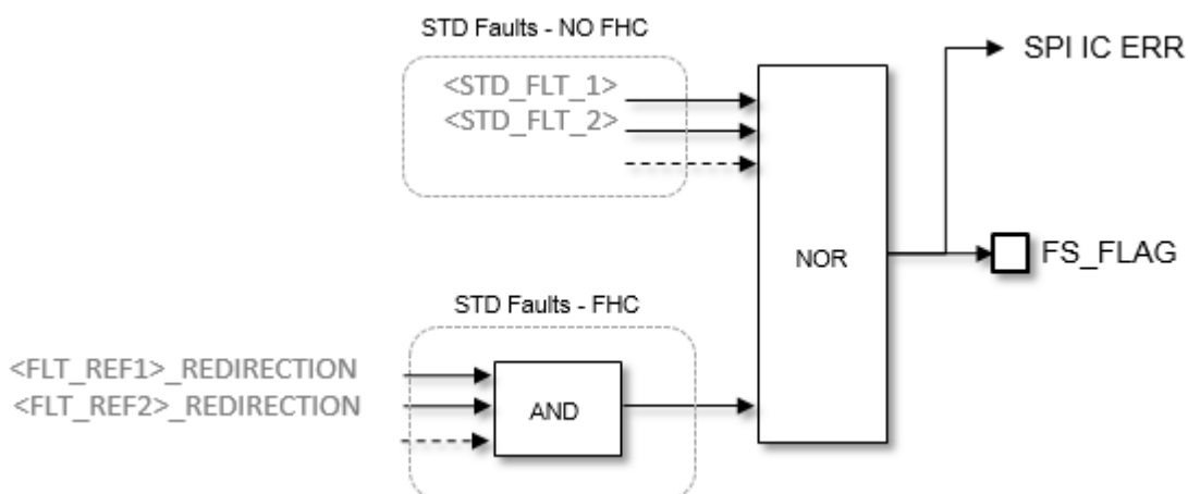
Figure 14. Fault output redirection logic simplified block diagram
