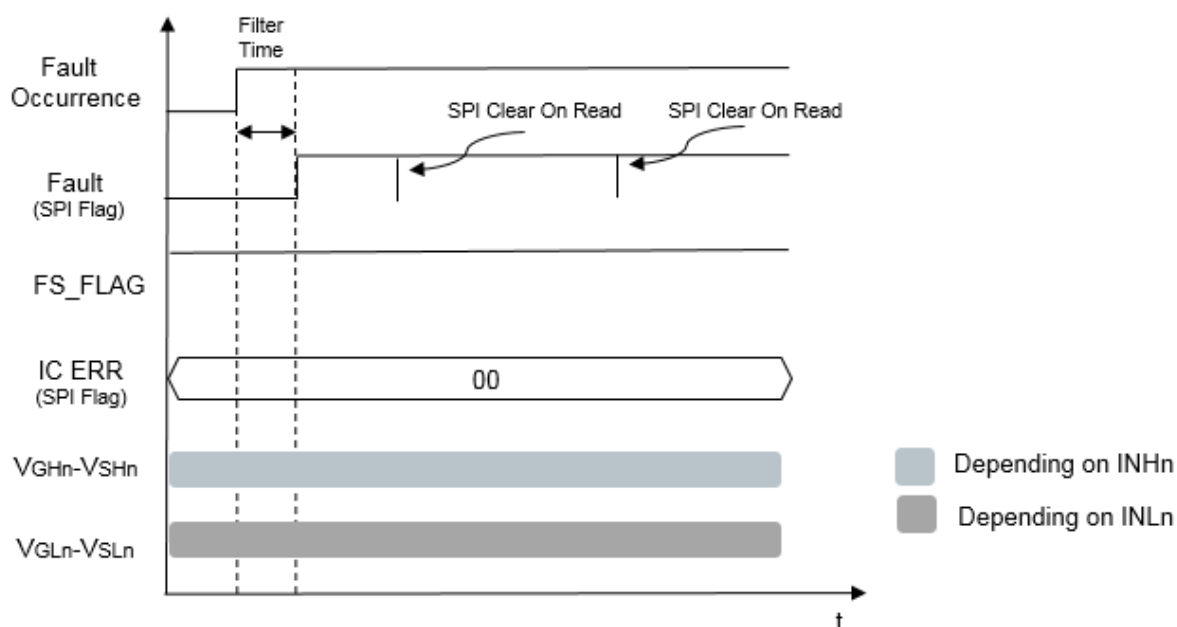
Figure 22. Warning - Permanent fault timing diagram
