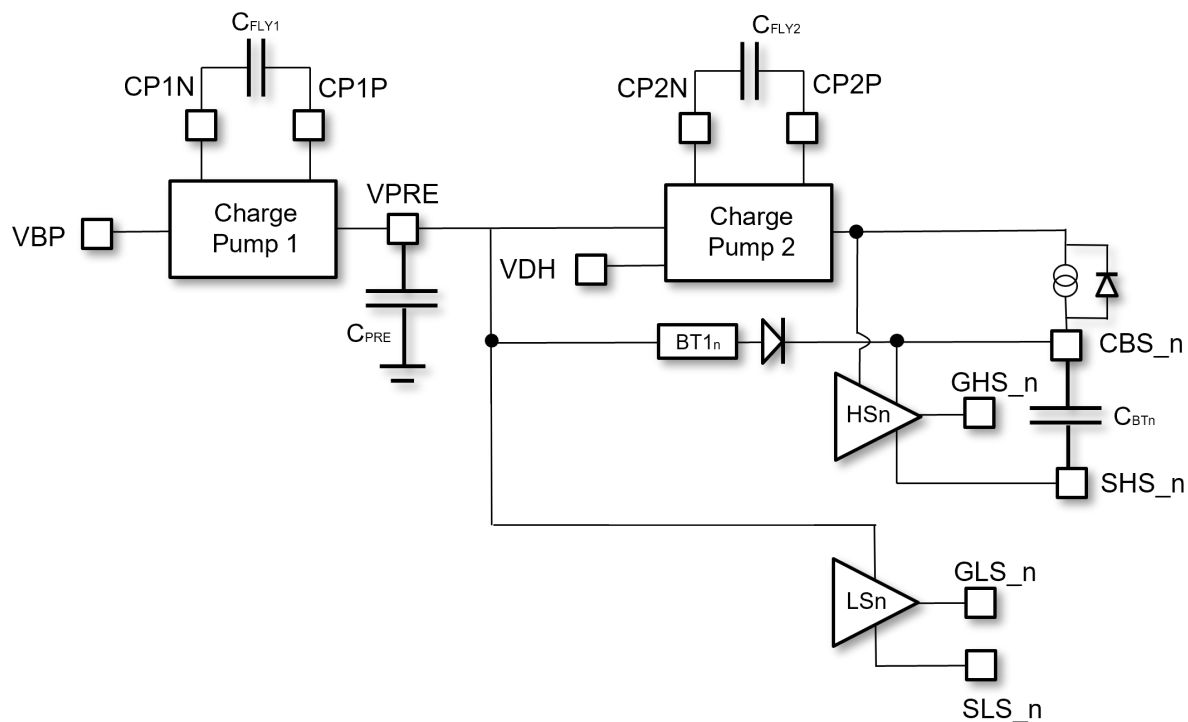
Figure 26. Ext. FET gate supply simplified block diagram
