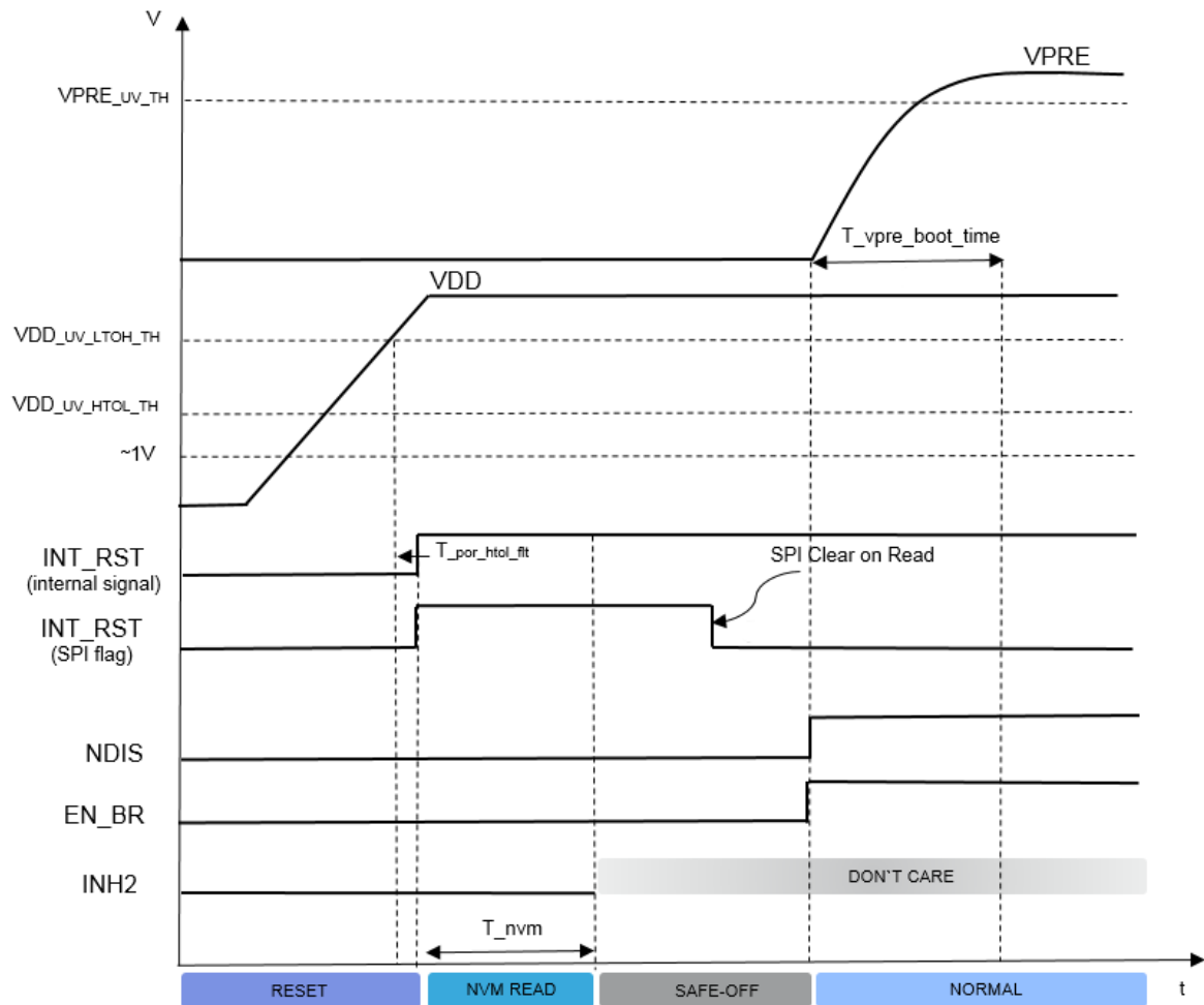
Figure 24. Recommended Power-Up sequence
