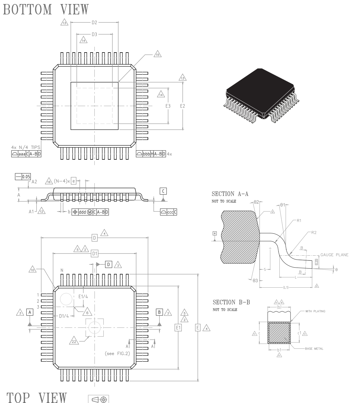
Figure 92. TQFP48 (7x7x1 mm exp. pad down) package outline
