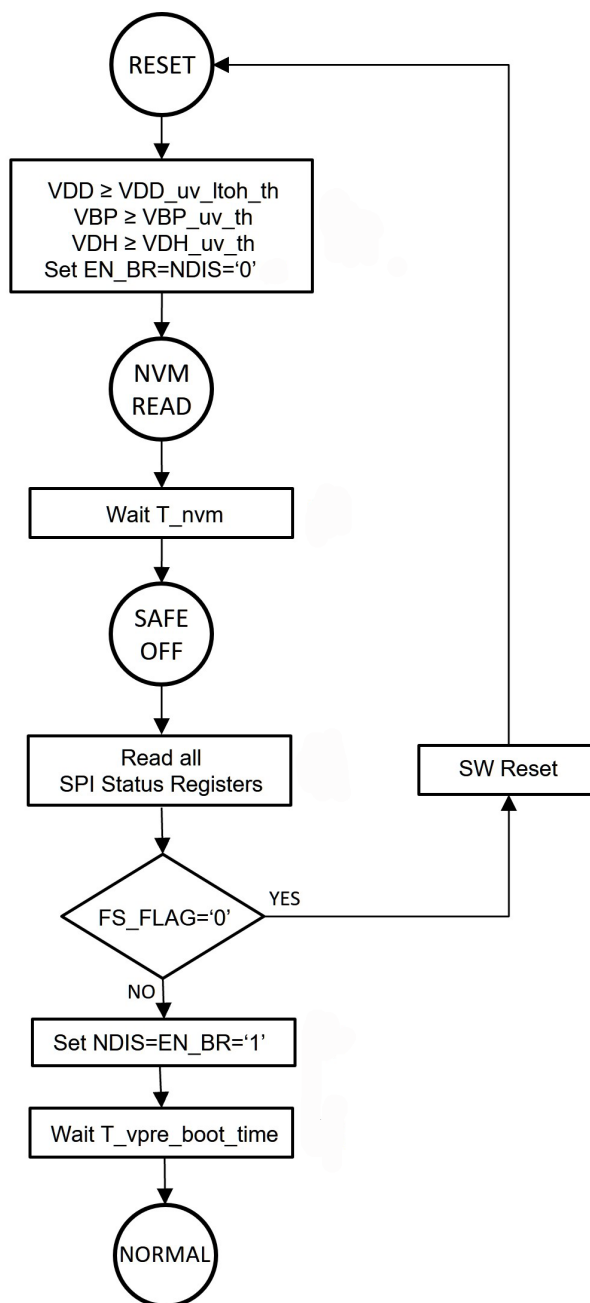
Figure 23. Power-Up diagram
