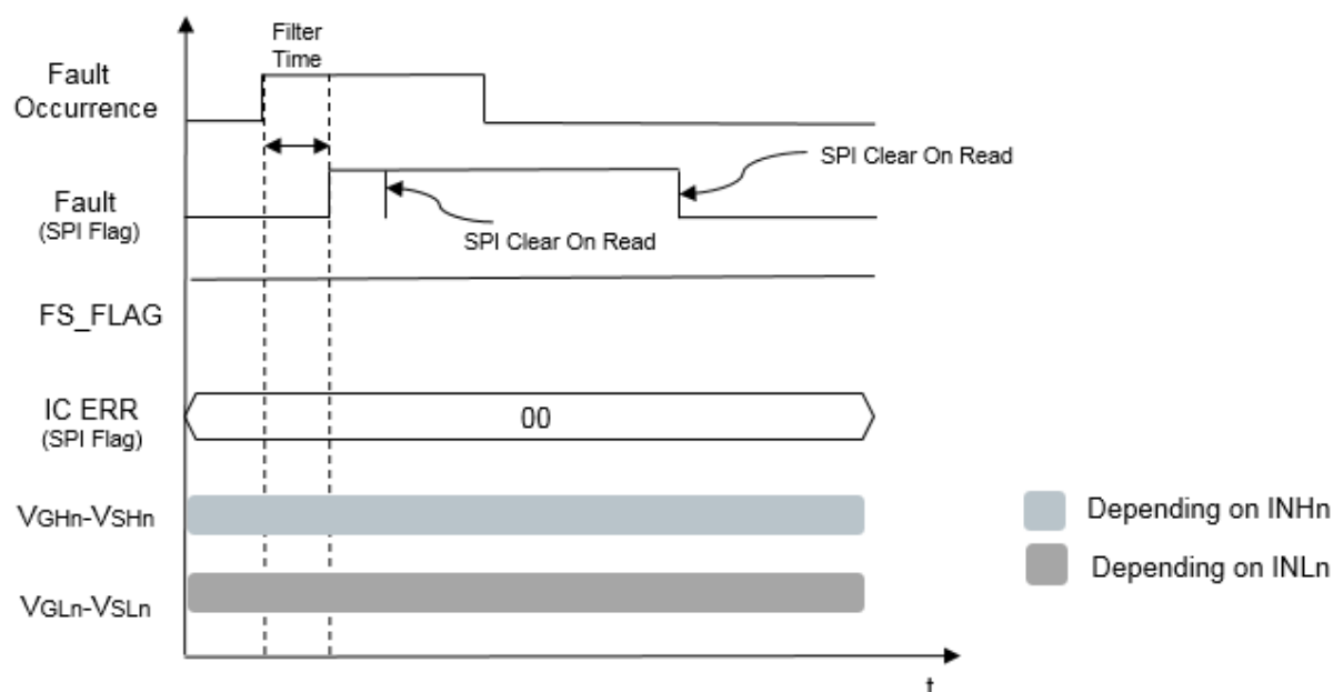
Figure 21. Warning - Transient fault timing diagram
