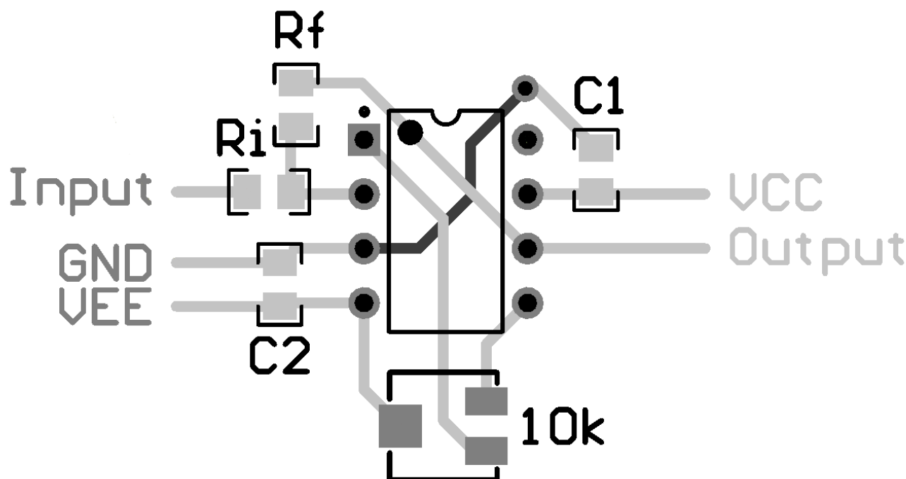
Figure 32. LF411-N Layout
