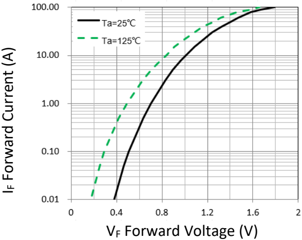
Figure 1. Forward Characteristic(typ.)
