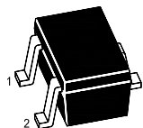
1.Base 2.Emitter 3.Collector SOT-323 Plastic Package
