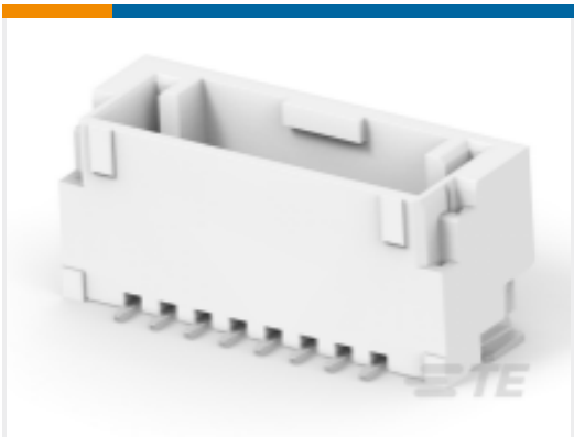
TE Part #2360540-8 SGI 1.25 HDR, 8P, VT, Key A, Natural
