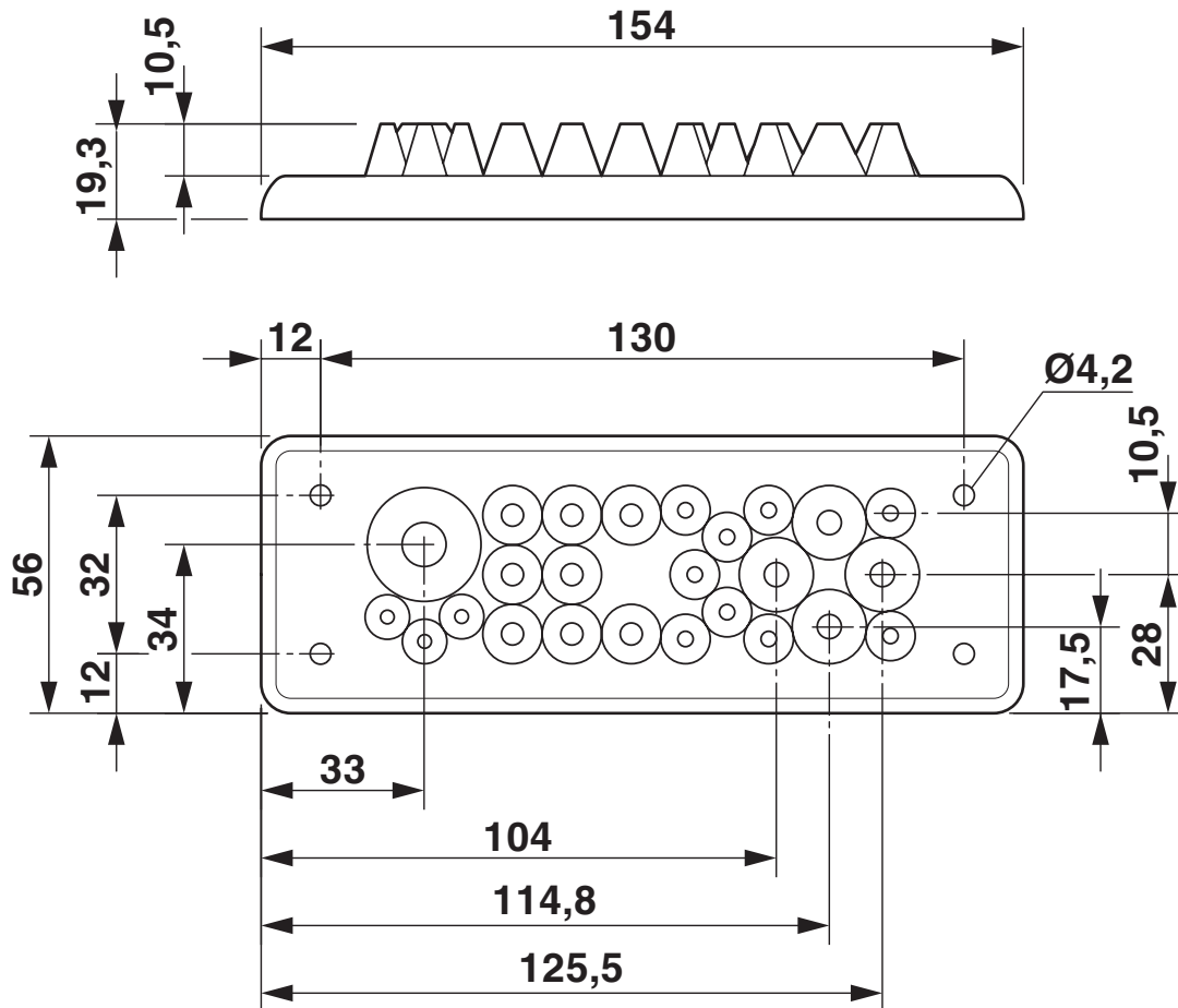
Dimensional drawing
