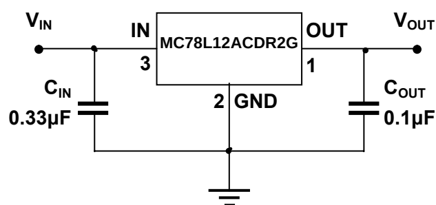
Conventional Circuit
