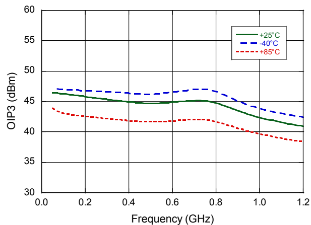
OIP3, P_{OUT} = +13\text{ dBm/ton}
