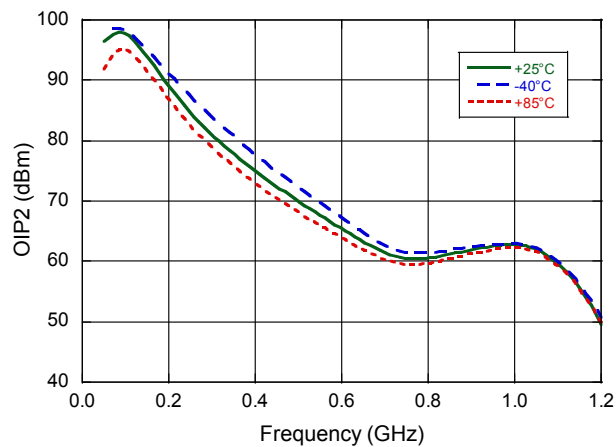
OIP2, P_{OUT} = +13\text{ dBm/ton}
