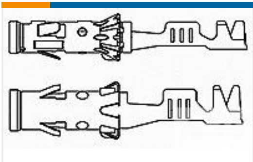
TE Part #929975-1 BU-KONTAKT 2,5MMD
