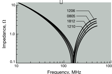
Variation of Impedance with Chip Size| Impedance vs. Frequency| 1000 pF - C0G (NP0) | 1206, 0805, 1812, 2512
