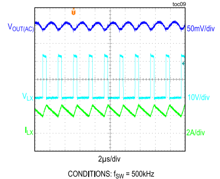
5V OUTPUT, STEADY-STATE AT 2.5A LOAD FIGURE 5 CIRCUIT
