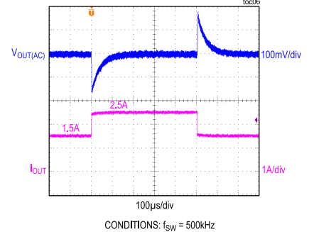
5V OUTPUT, LOAD TRANSIENT BETWEEN 1.5A AND 2.5A FIGURE 5 CIRCUIT
