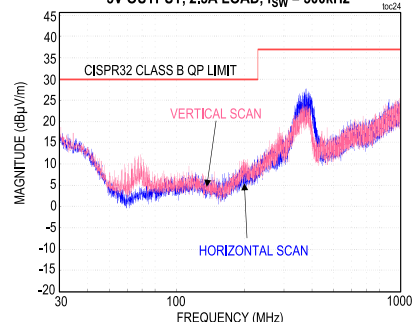
MAX17783C RADIATED EMISSIONS PLOT, 5V OUTPUT, 2.5A LOAD, f_{SW} = 500kHz
