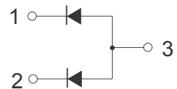
SOT-23 (TO-236-3)
