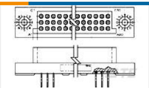
TE Part #448006-1 3 ROW BOX RECP 120 POS
