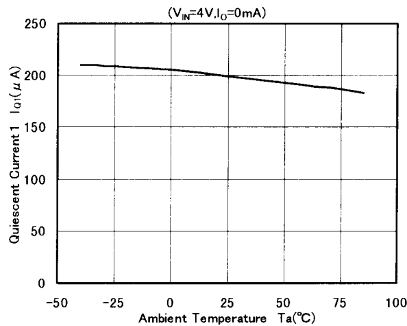
NJM2370 3V Version Quiescent Current 1 vs. Ambient Temperature ( V_{IN}=4\text{V}, I_O=0\text{mA} )
