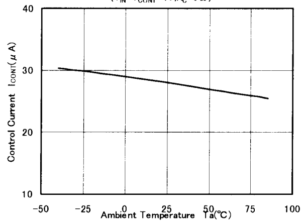
NJM2370 3V Version Control Current vs. Ambient Temperature ( V_{IN}=V_{CONT}=4\text{V}, R_C=0\Omega )
