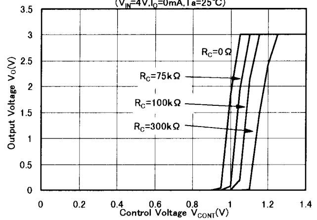
NJM2370 3V Version Output Voltage vs. Control Voltage ( V_{IN}=4V, I_O=0mA, T_a=25^\circ C )
