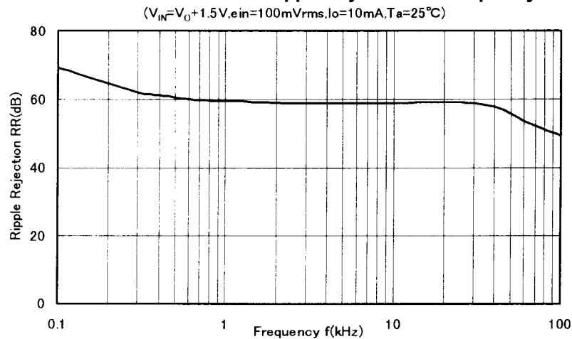
NJM2370 3V Version Ripple Rejection vs. Frequency
