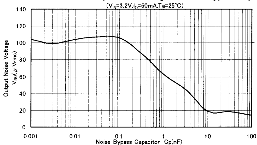
NJM2370 3V Version Output Noise Voltage vs. Noise Bypass Capacitor
