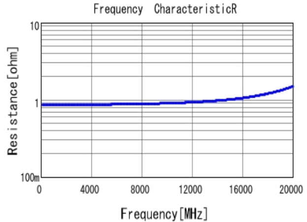
■ GRM0335C1HR60BA01 R DC0V, 25degC
