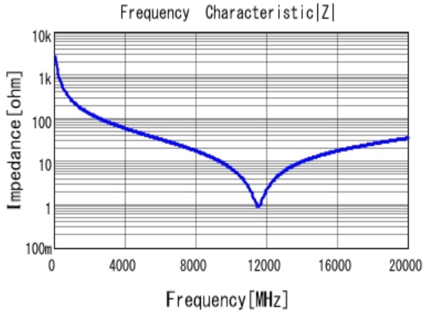
■ GRM0335C1HR60BA01 |Z| DC0V, 25degC
