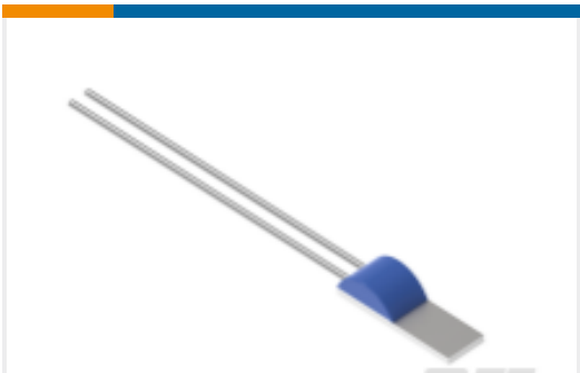
TE Part #NB-PTCO-012 Pt1000, 1.2x4.0, Class B, PTFM102B1G0
