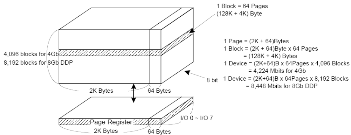
Figure 3.2 Array Organization(x8)
