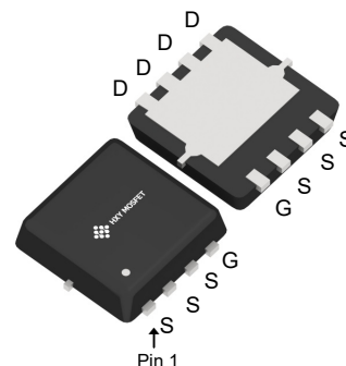
DFN3X3-8L DFN-8(3x3)
