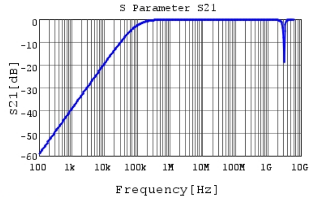
KRM55L5C2J183JDL1 S21 DCOV, 25degC
