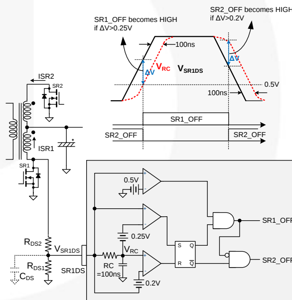
Figure 79. SR Conduction Detection with Single Pin (SR1DS Pin)
