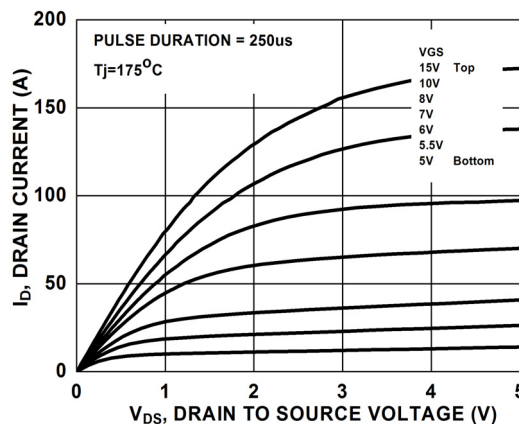
Figure 10. Saturation Characteristics
