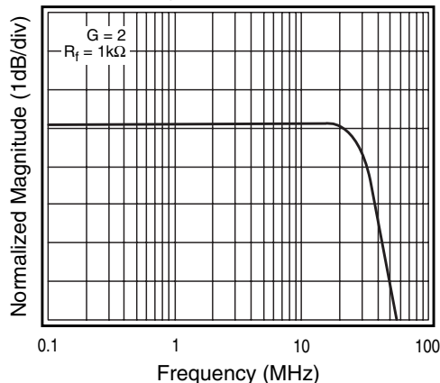
Non-Inverting Freq. Response V_s = +5V
