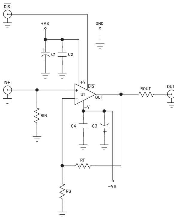
Figure 6: Evaluation Board Schematic
