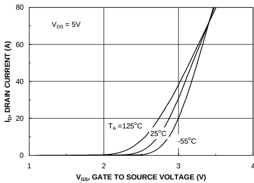
Figure 5. Transfer Characteristics
