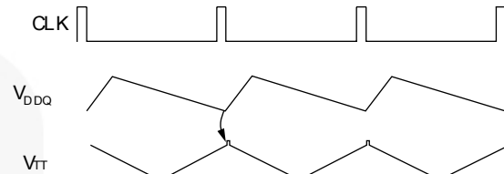
Figure 7. Noise-Susceptible 180° Phasing for DDR1
