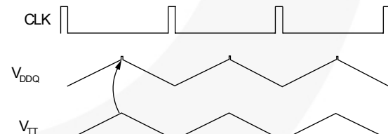
Figure 9. Noise-Susceptible In-Phase Operation for DDR2
