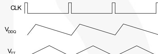
Figure 8. Optimal In-Phase Operation for DDR1
