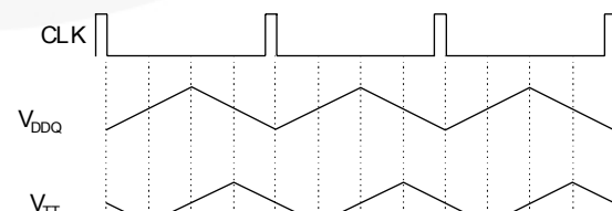
Figure 10. Optimal 90° Phasing for DDR2
