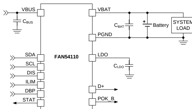
Figure 1. Typical Application
