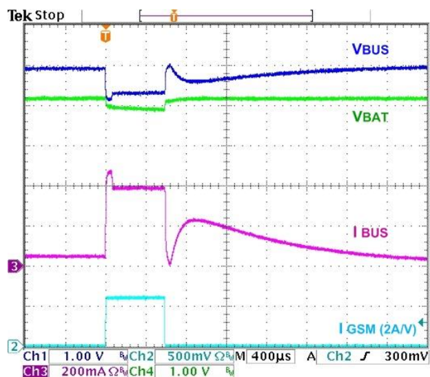
Figure 18. 1.2\text{ A} Load Pulse, t_r=t_f=5\text{ }\mu\text{s} , 500\text{ mA} Current Limited Source, 4.2\text{ V}_{\text{BAT}} , 1.0\text{ A } I_{\text{OCHRG}} , 4.32\text{ V}_{\text{BUS\_REF}}
