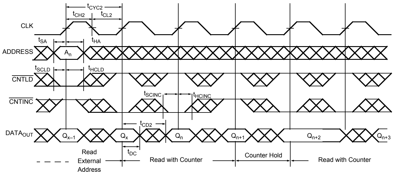
Figure 8. Read with Address Counter Advance [23, 24]
