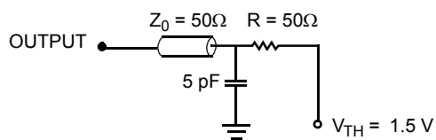
Figure 2. AC Test Load
