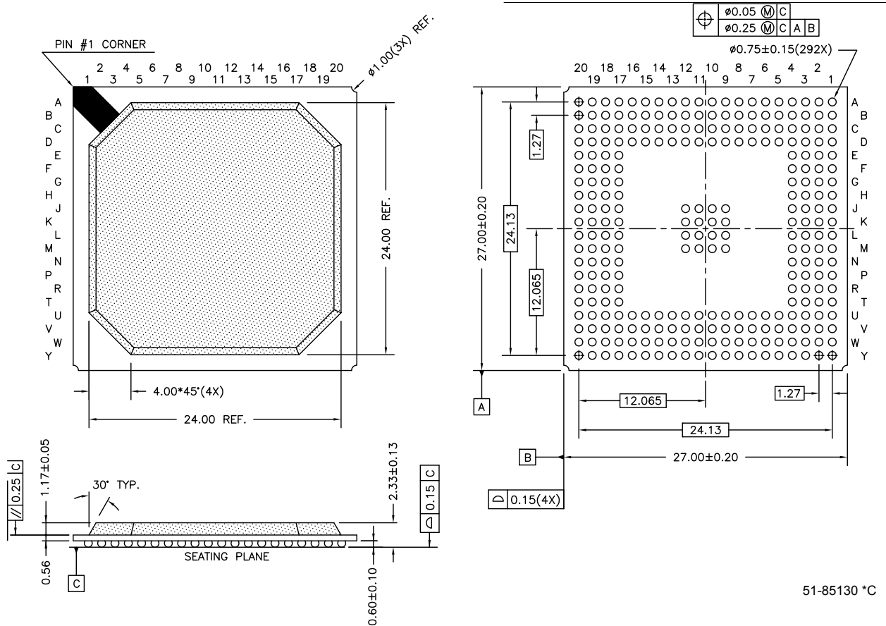
Figure 19. 272-ball PBGA (27 × 27 × 2.33 mm) BG272
