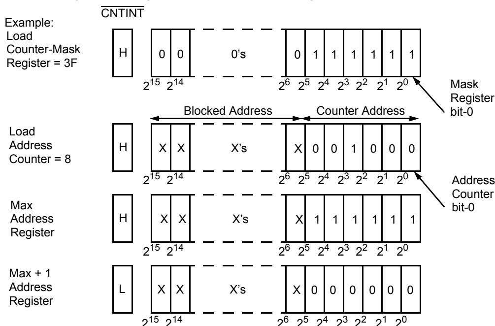
Figure 17. Programmable Counter-Mask Register Operation [53]
