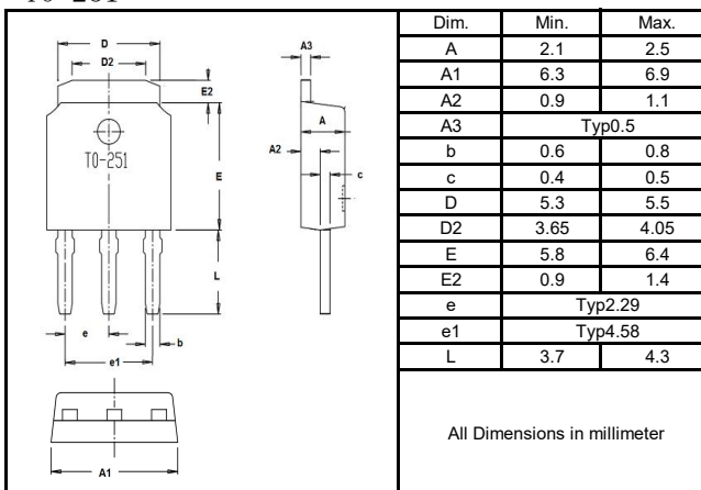
T0-251
