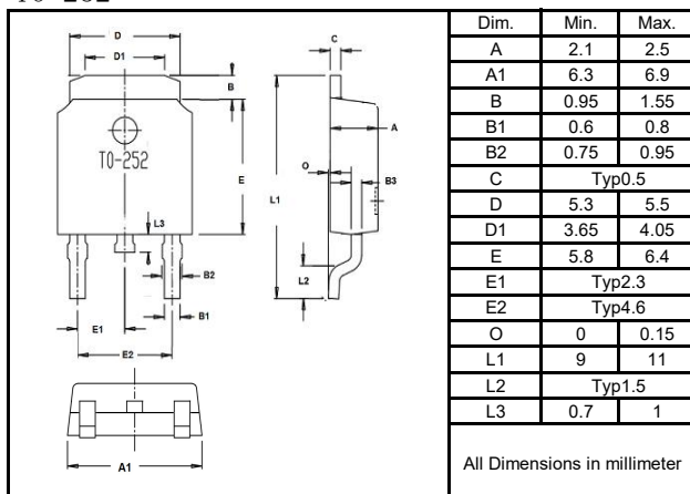
T0-252
