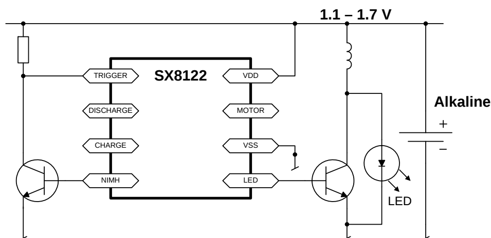
Figure 8. LED is continuously on when the supply voltage is below NiMH threshold
